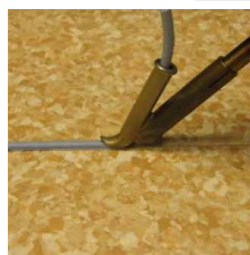
Welding PVC and Linoleum
