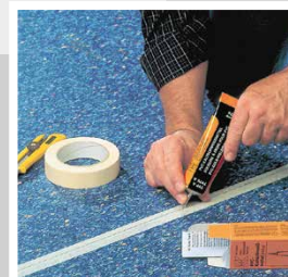
Welding PVC and Linoleum
