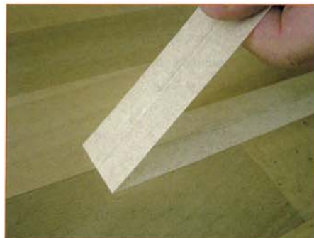
After approx. 10 minutes pull off the masking tape backwards at an angle.
